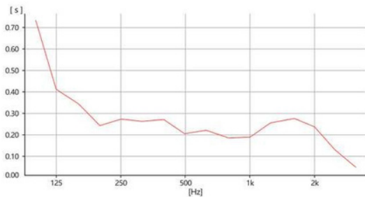
Reverberation time test
