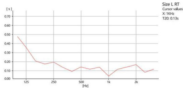
Reverberation time test
