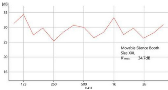
Sound insulation test
