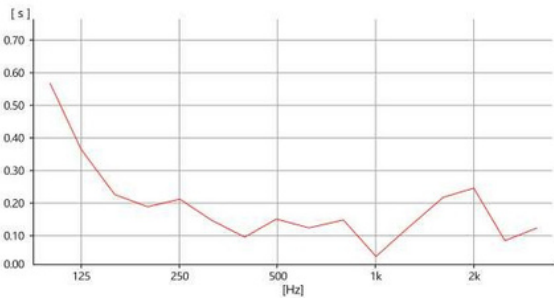
Reverberation time test
