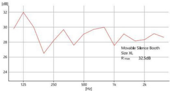
Sound insulation test
